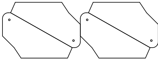
15 CONTROL HORN 4 PLASTIC CARD AP EAZY DUCTED FAN - V0.2
