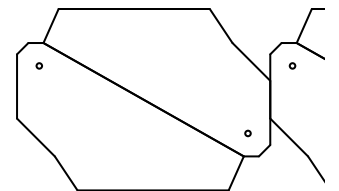
BC8 CONTROL HORN (AILERON) 4 PLASTIC CARD AP GODAI - VERSION 1.0
