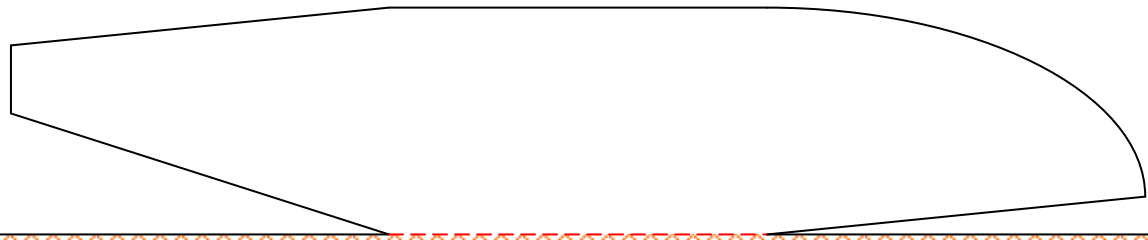
24.a SIDE PONTOON PYLON SUPPORT 2 FOAM BOARD AP KWAK - PONTOON UPGRADE - V1.0
